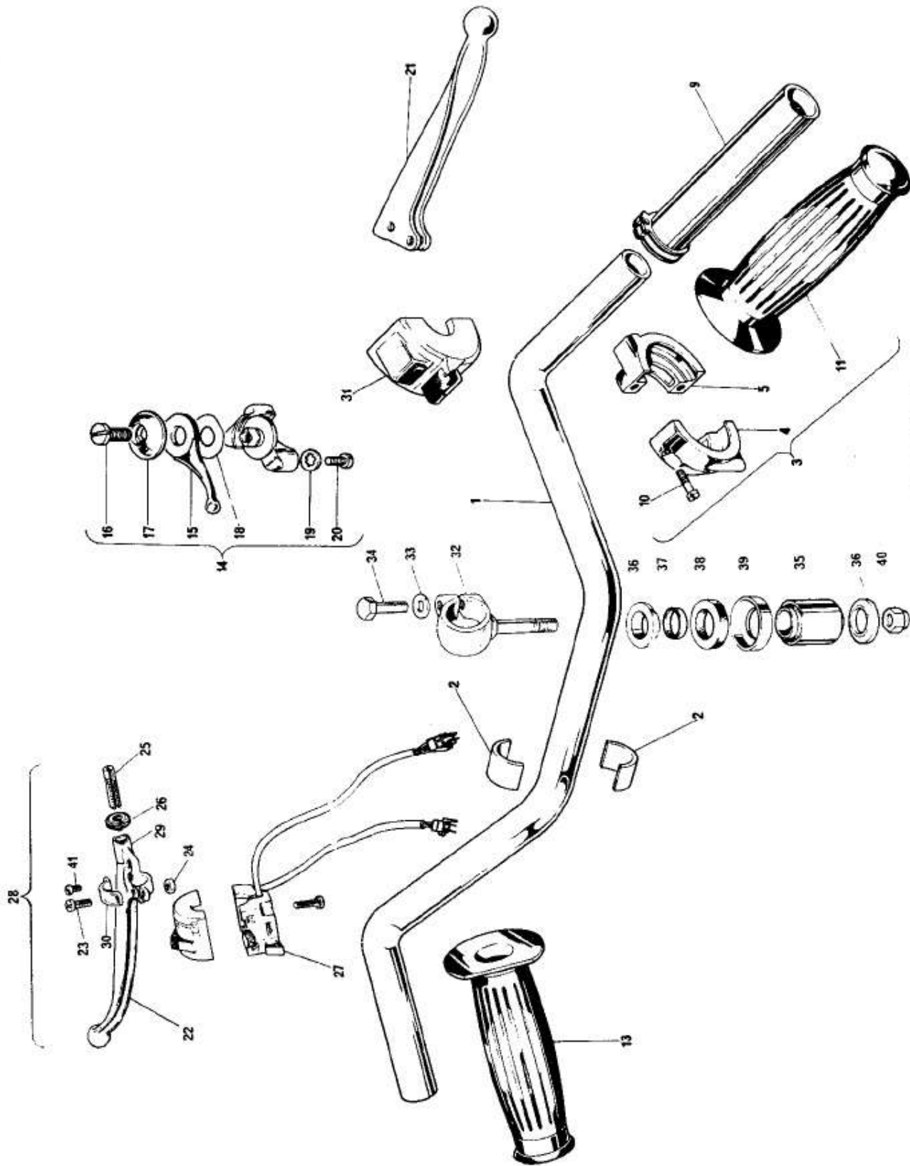
Fig. 29. HANDLEBAR AND CONTROL LEVERS
