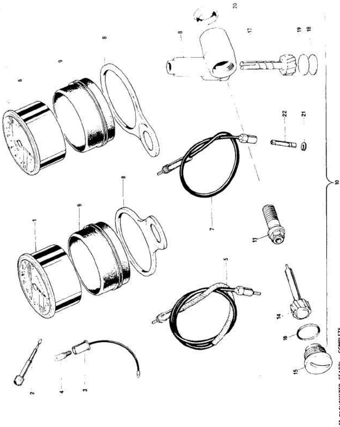
Fig. 32. SPEEDOMETER AND TACHOMETER
