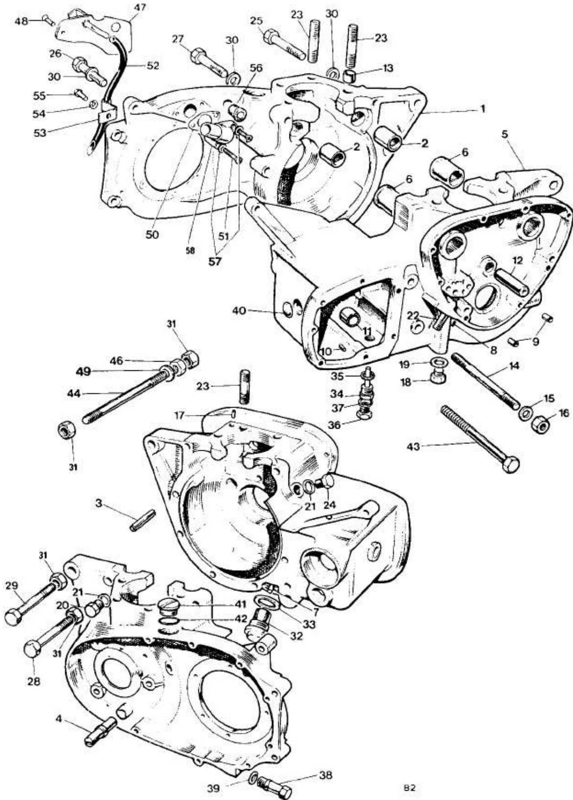
Fig. 2 CRANKCASE
