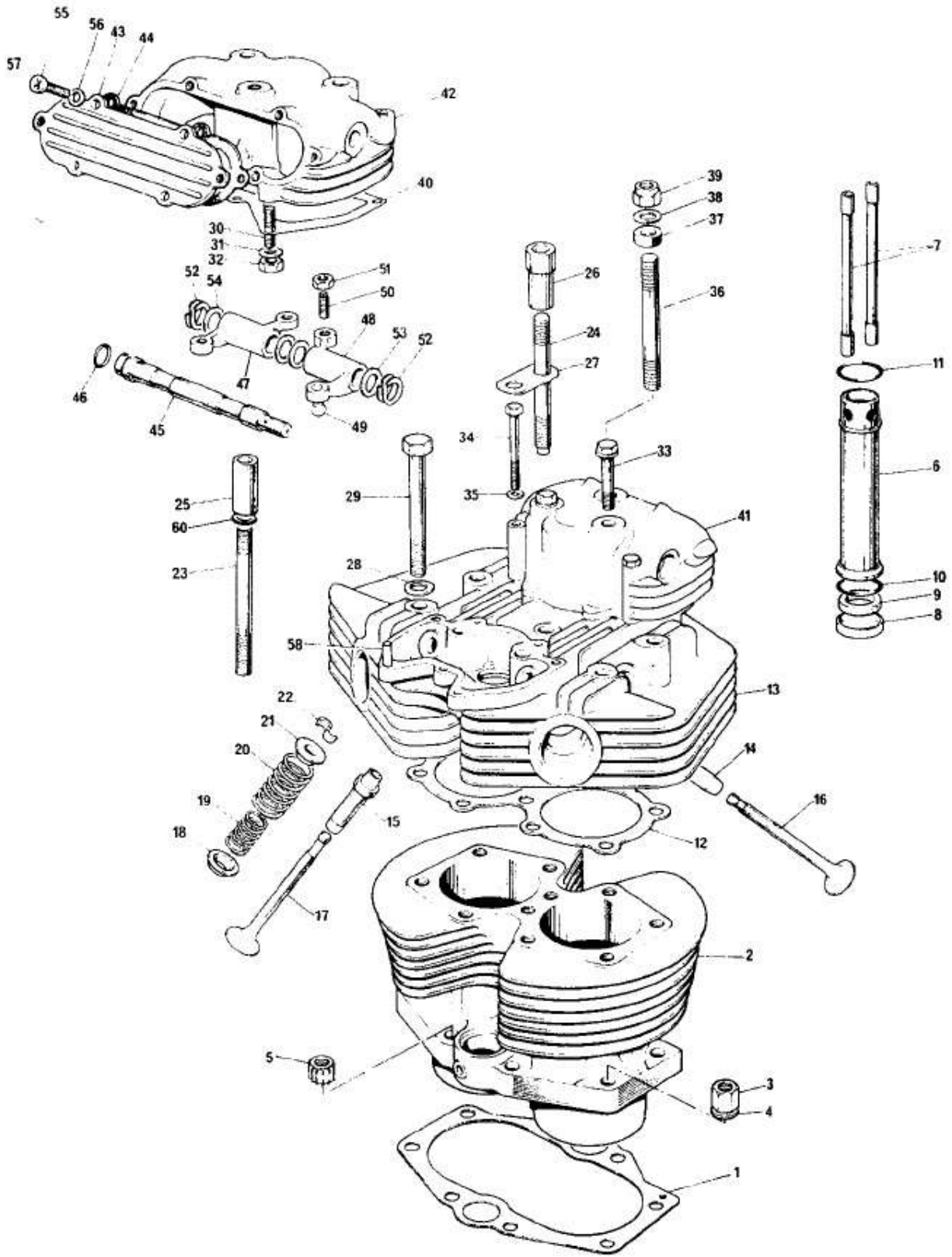
CYLINDER BLOCK & HEAD, T140V
