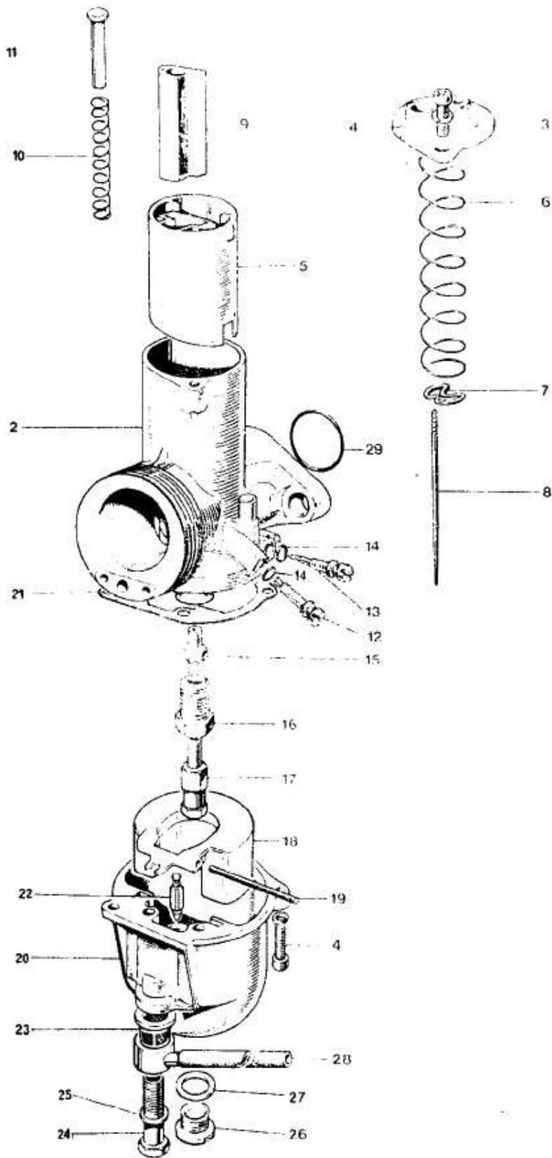
Fig.9. AMAL CARBURETOR, T140V
