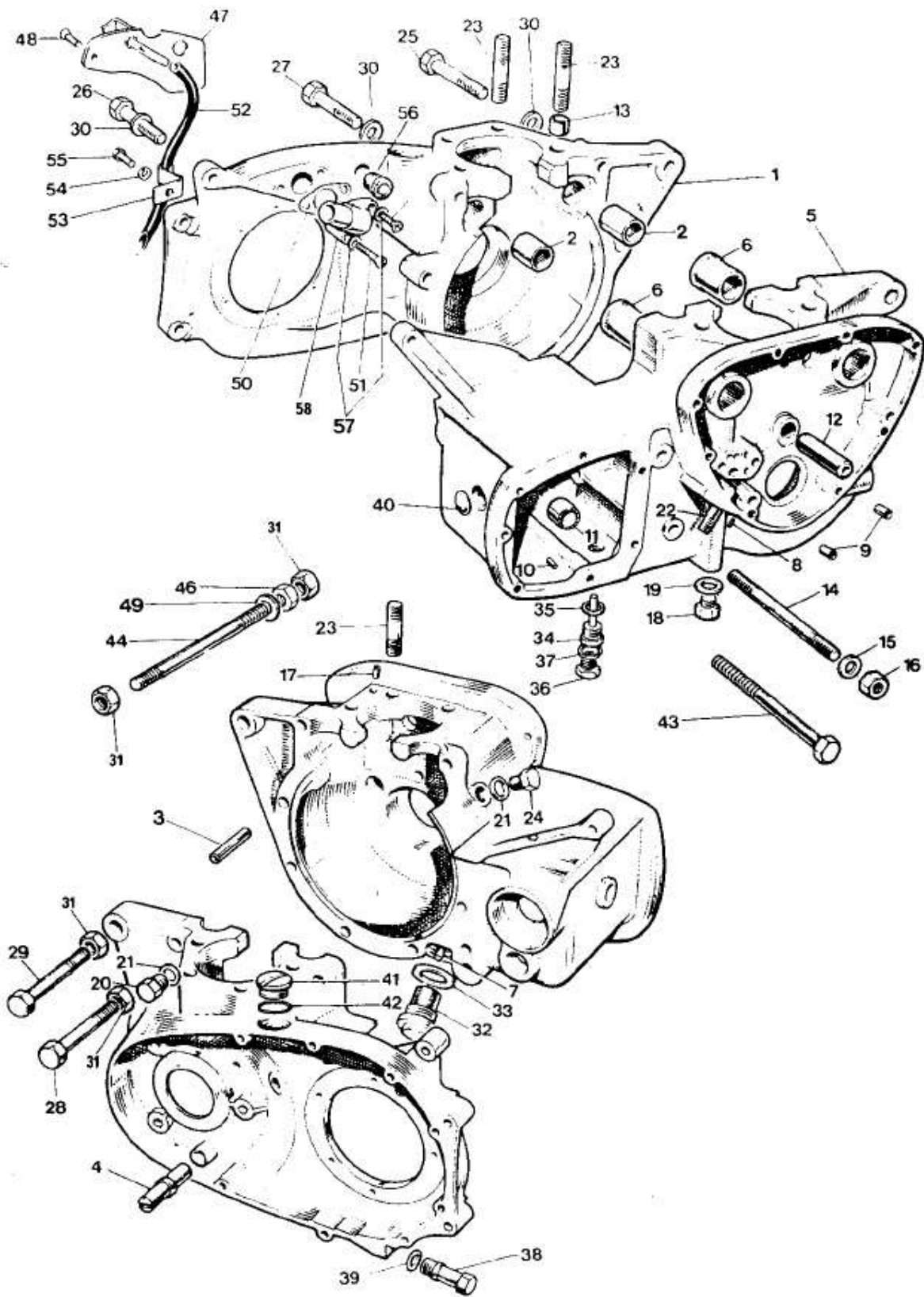
Fig. 2 CRANKCASE
